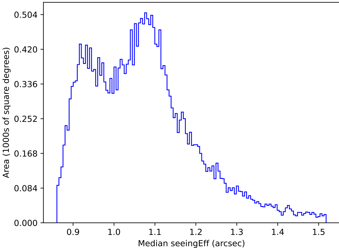
too_elab_r8_d3_griz_v3.4_10yrs All sky r band: Median seeingEff
