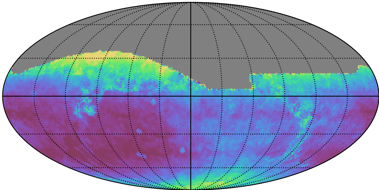
too_elab_r8_d3_griz_v3.4_10yrs All sky i band: Median seeingEff
