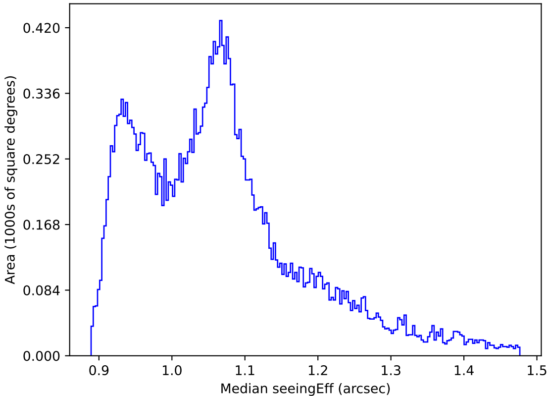
too_elab_r8_d3_griz_v3.4_10yrs All sky all bands: Median seeingEff
