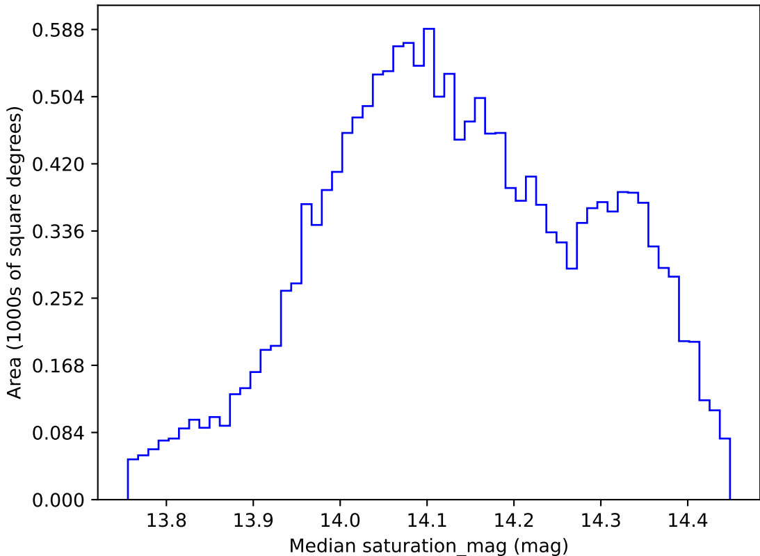
too_elab_r8_d3_griz_v3.4_10yrs WFD z band: Median saturation_mag
