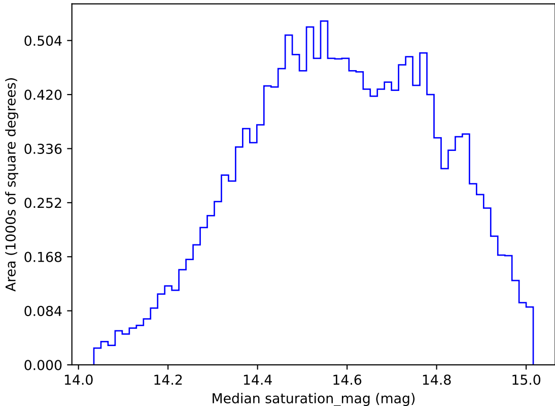
too_elab_r8_d3_griz_v3.4_10yrs WFD g band: Median saturation_mag
