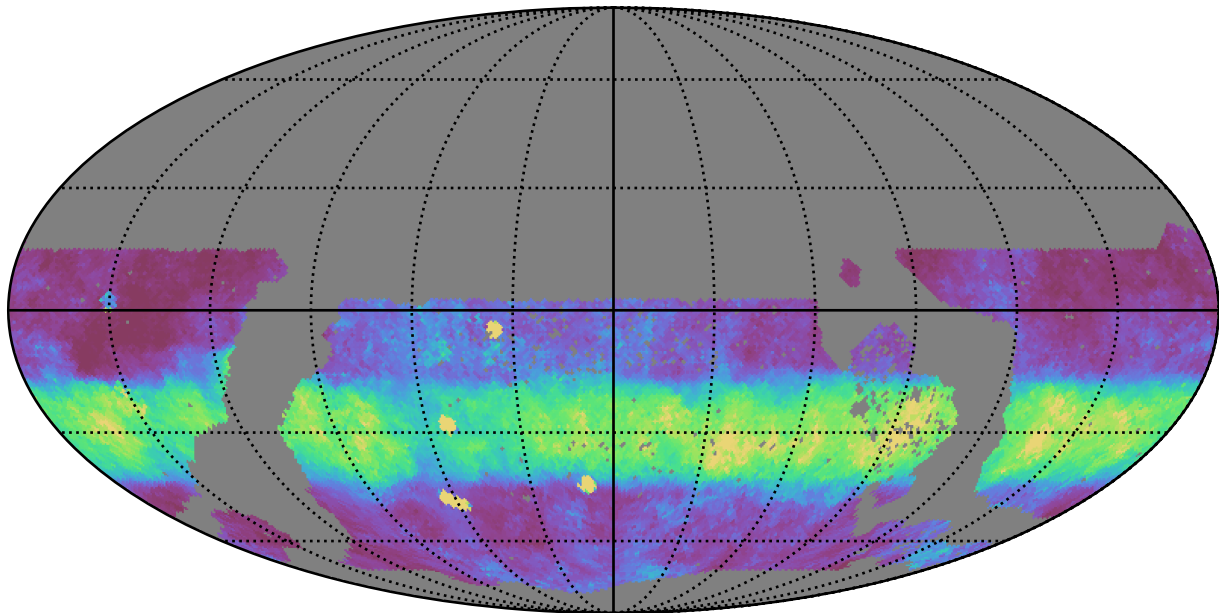
too_elab_r8_d3_griz_v3.4_10yrs WFD z band: Median normairmass
