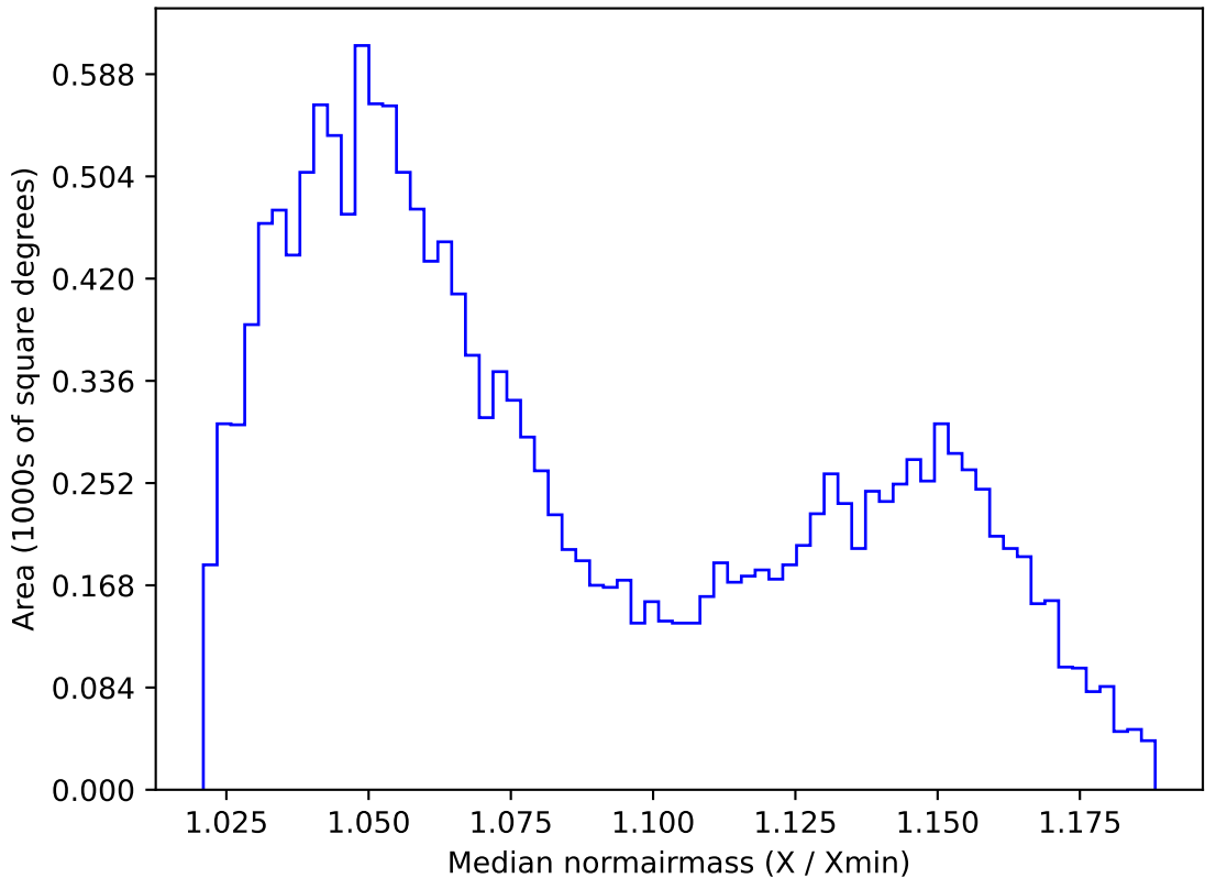
too_elab_r8_d3_griz_v3.4_10yrs WFD z band: Median normairmass
