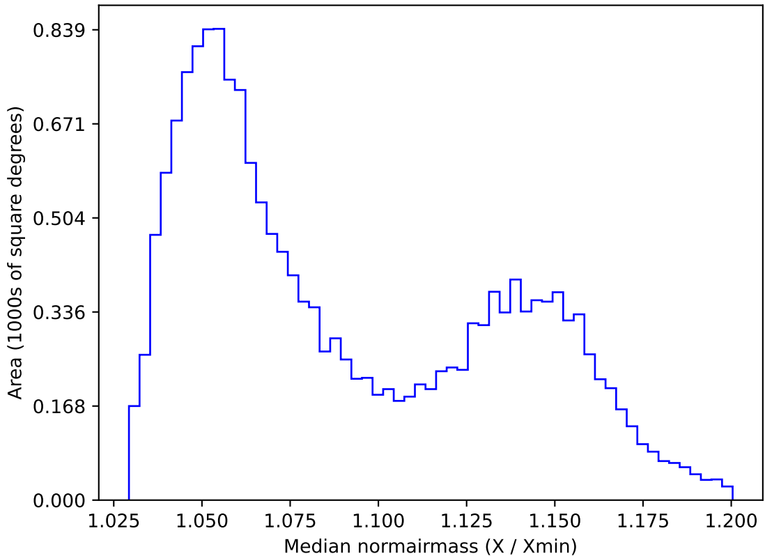
too_elab_r8_d3_griz_v3.4_10yrs WFD y band: Median normairmass
