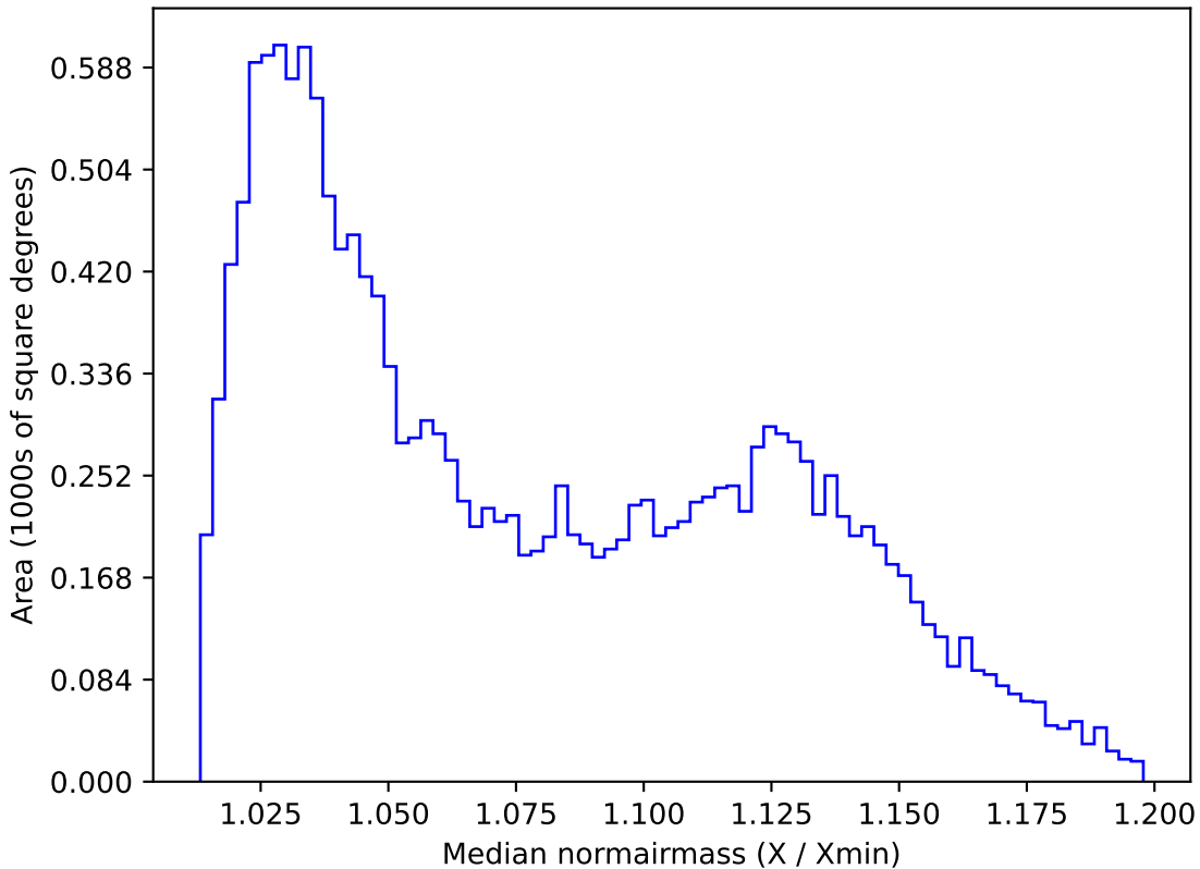
too_elab_r8_d3_griz_v3.4_10yrs WFD u band: Median normairmass
