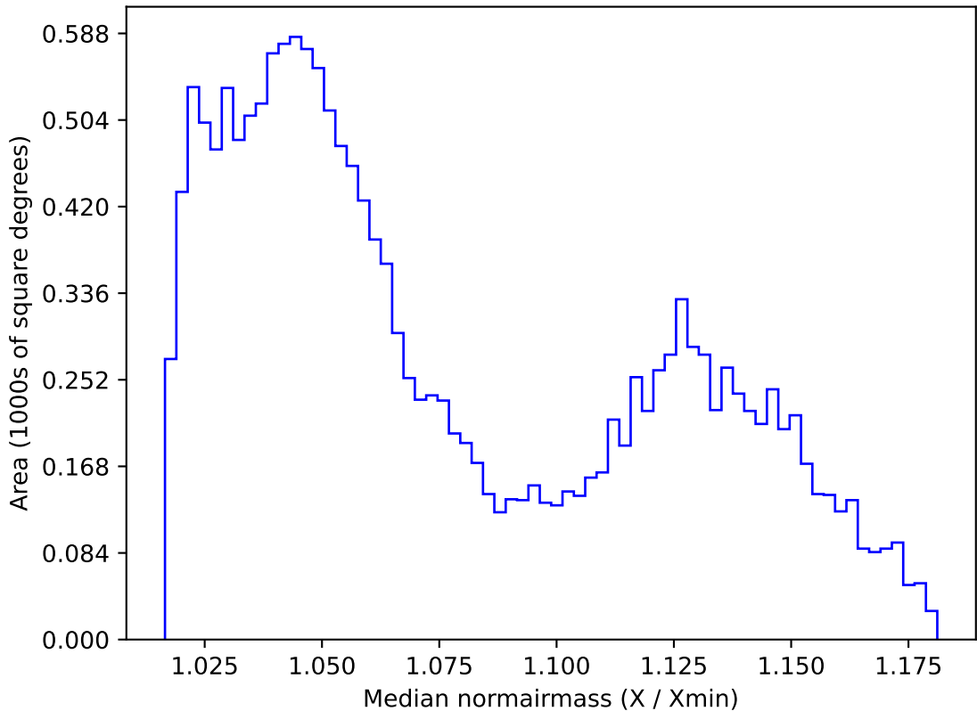
too_elab_r8_d3_griz_v3.4_10yrs WFD r band: Median normairmass
