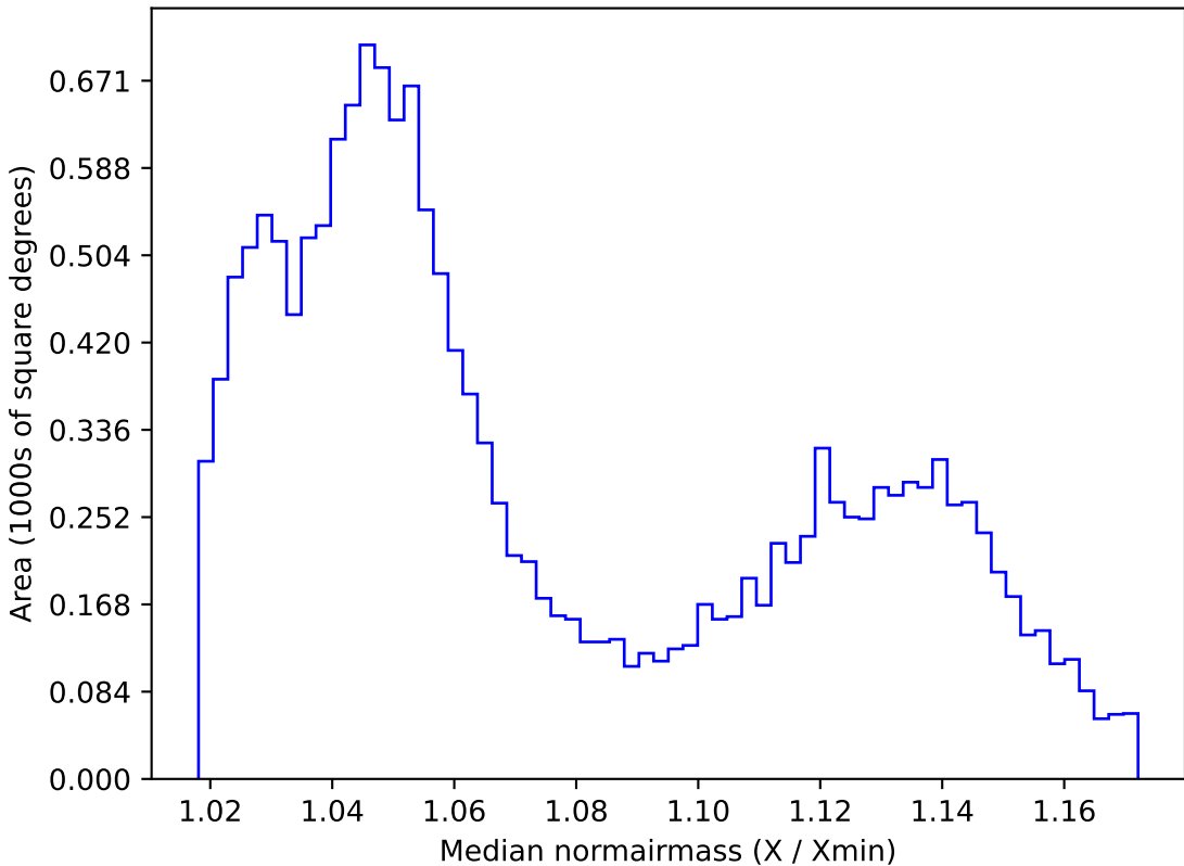
too_elab_r8_d3_griz_v3.4_10yrs WFD i band: Median normairmass
