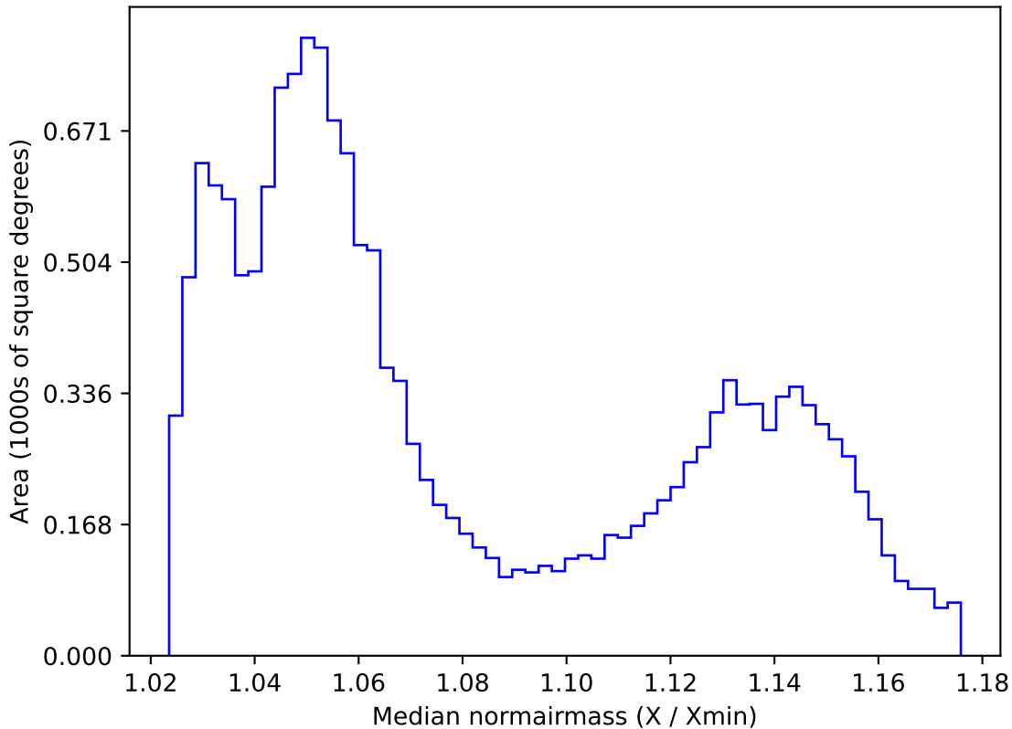
too_elab_r8_d3_griz_v3.4_10yrs WFD all bands: Median normairmass
