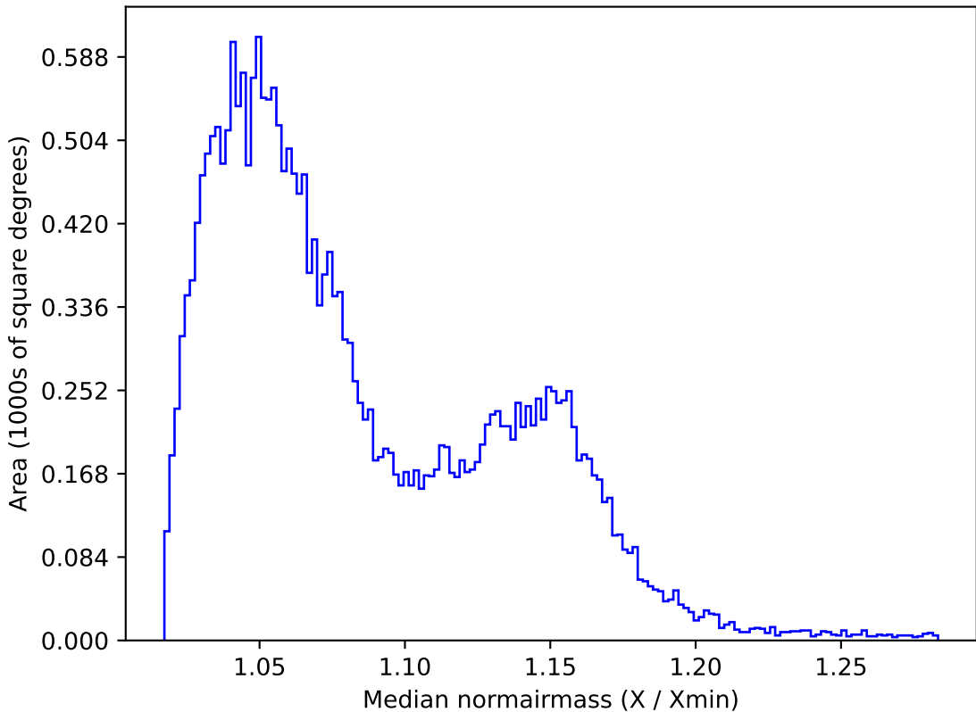
too_elab_r8_d3_griz_v3.4_10yrs All sky z band: Median normairmass
