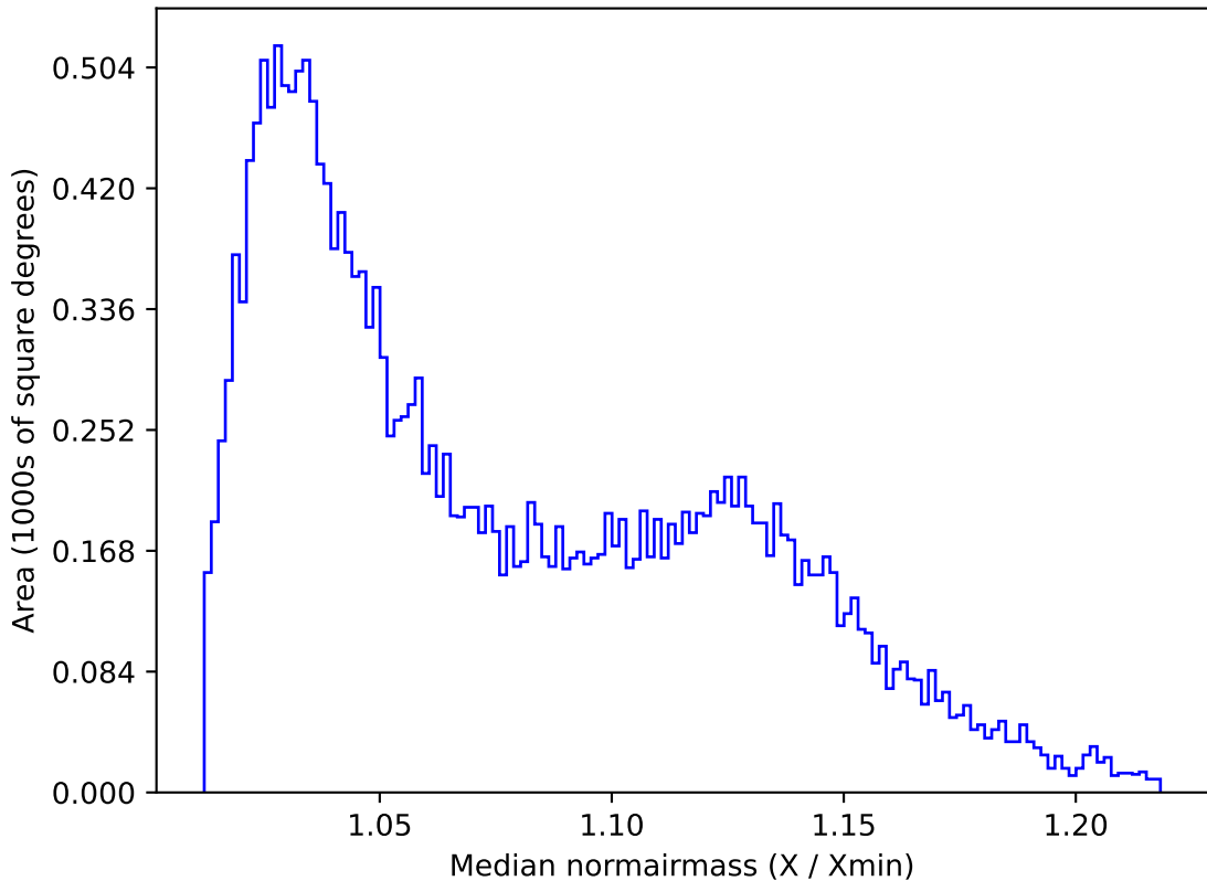
too_elab_r8_d3_griz_v3.4_10yrs All sky u band: Median normairmass
