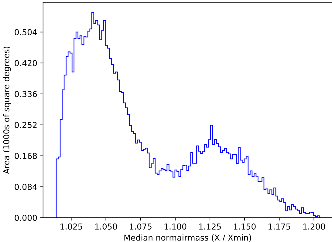
too_elab_r8_d3_griz_v3.4_10yrs All sky r band: Median normairmass
