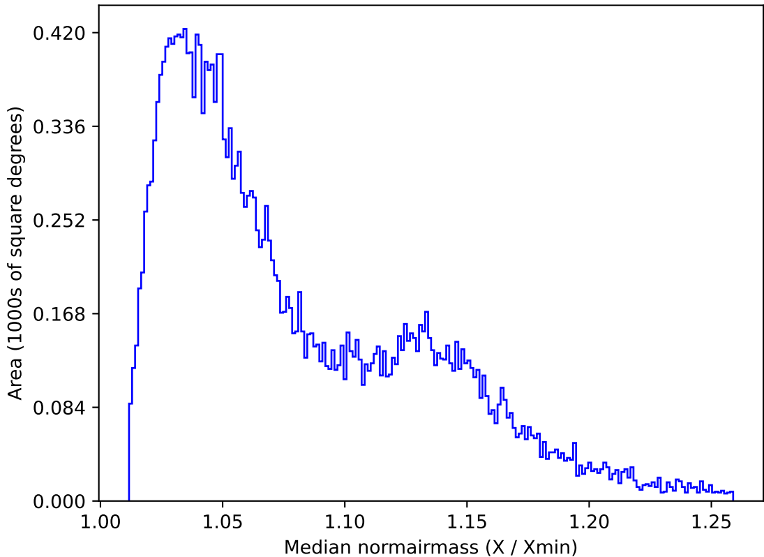
too_elab_r8_d3_griz_v3.4_10yrs All sky g band: Median normairmass
