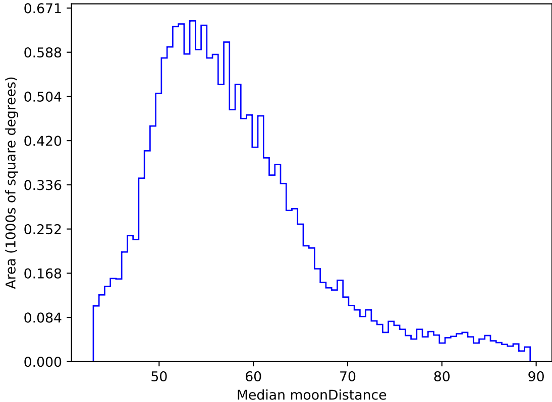
too_elab_r8_d3_griz_v3.4_10yrs WFD y band: Median moonDistance
