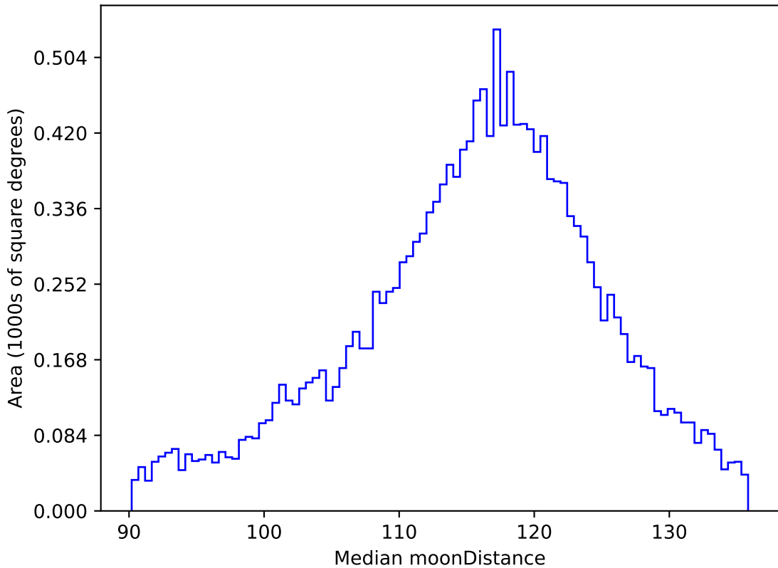
too_elab_r8_d3_griz_v3.4_10yrs WFD g band: Median moonDistance
