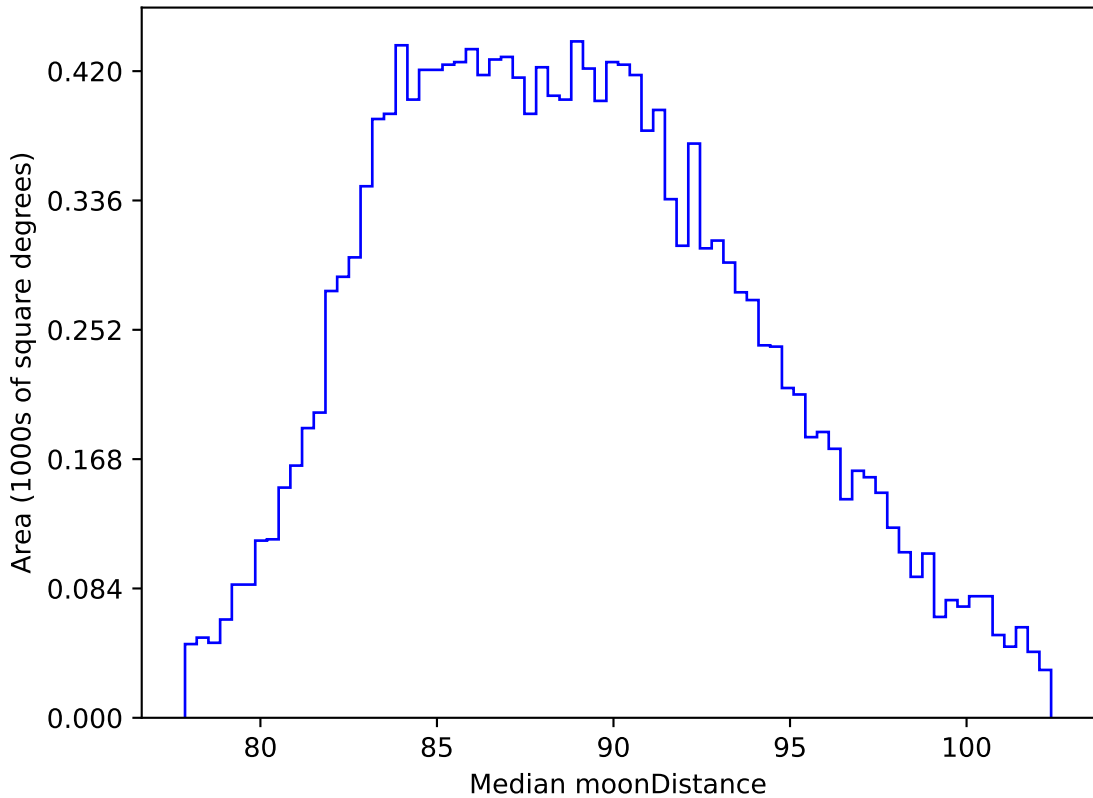
too_elab_r8_d3_griz_v3.4_10yrs WFD all bands: Median moonDistance
