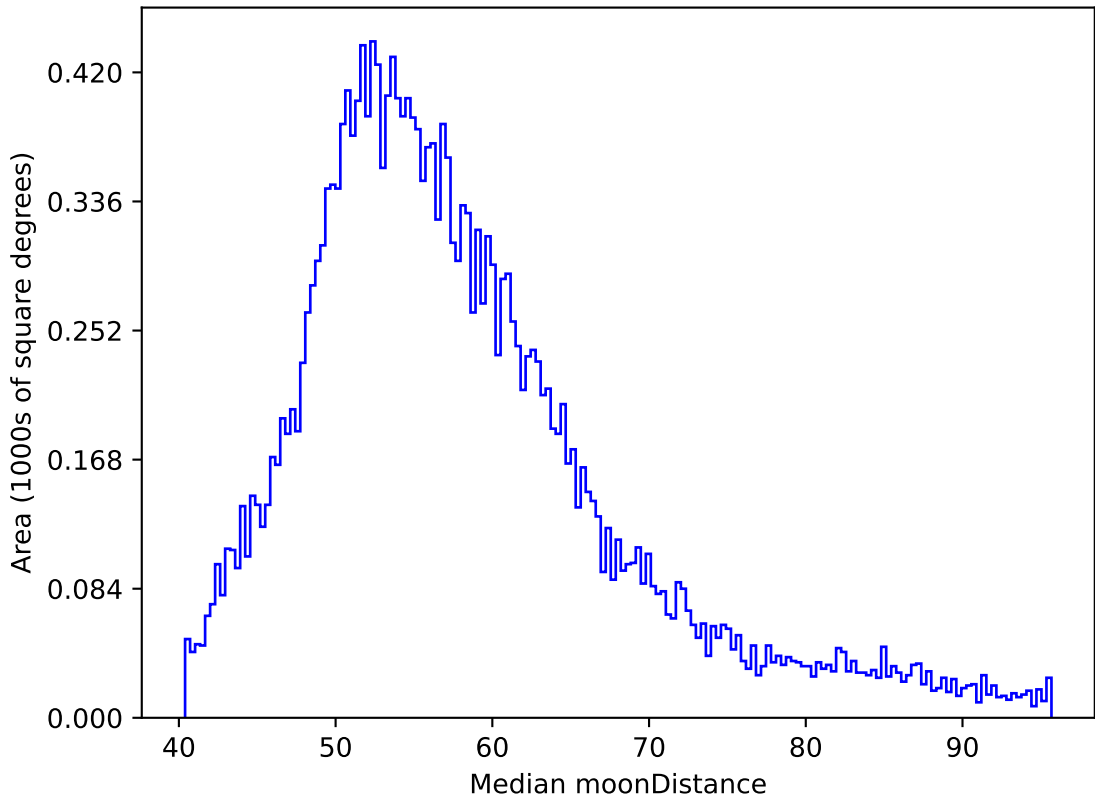
too_elab_r8_d3_griz_v3.4_10yrs All sky y band: Median moonDistance
