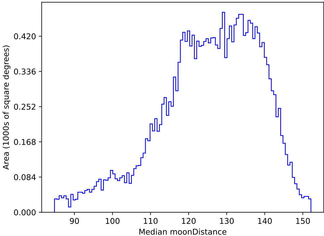
too_elab_r8_d3_griz_v3.4_10yrs All sky u band: Median moonDistance
