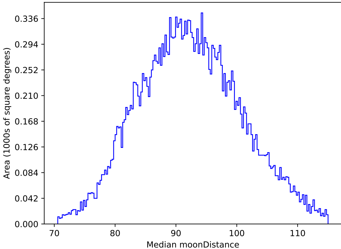
too_elab_r8_d3_griz_v3.4_10yrs All sky i band: Median moonDistance
