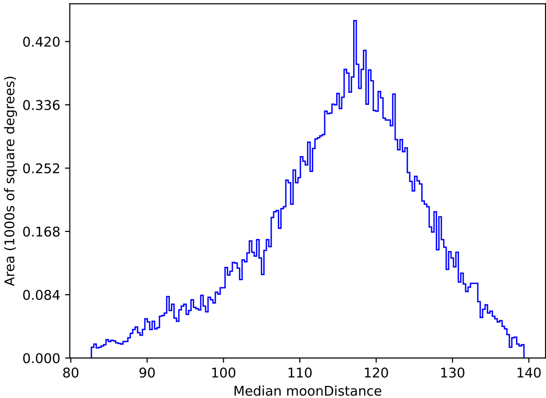
too_elab_r8_d3_griz_v3.4_10yrs All sky g band: Median moonDistance
