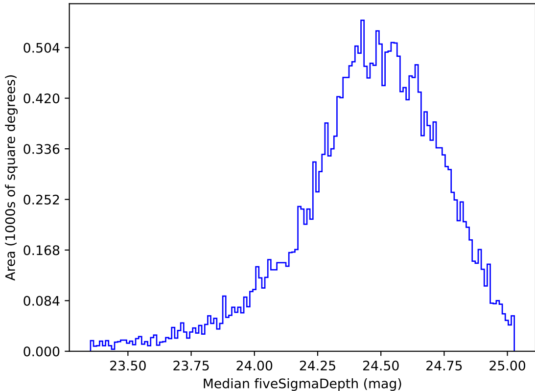
too_elab_r8_d3_griz_v3.4_10yrs Yr 1 g band: Median fiveSigmaDepth
