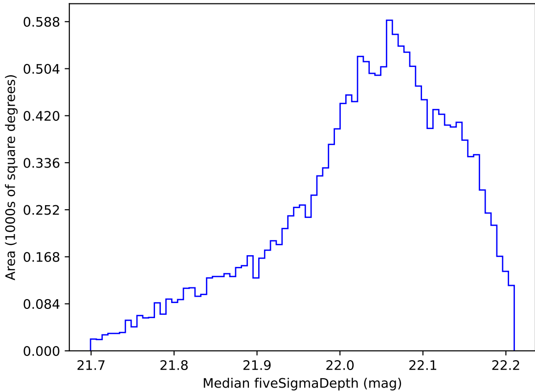
too_elab_r8_d3_griz_v3.4_10yrs WFD y band: Median fiveSigmaDepth
