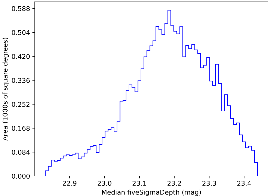
too_elab_r8_d3_griz_v3.4_10yrs WFD u band: Median fiveSigmaDepth
