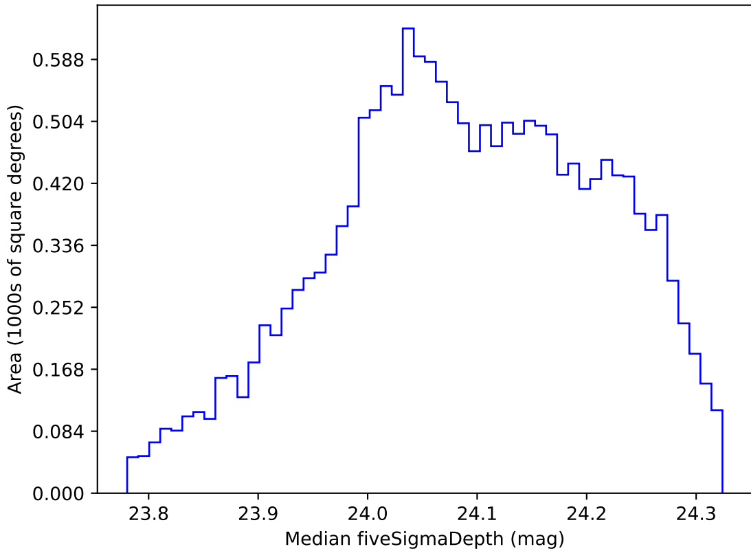
too_elab_r8_d3_griz_v3.4_10yrs WFD r band: Median fiveSigmaDepth
