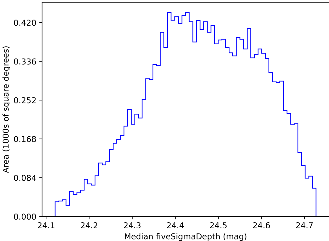
too_elab_r8_d3_griz_v3.4_10yrs WFD g band: Median fiveSigmaDepth
