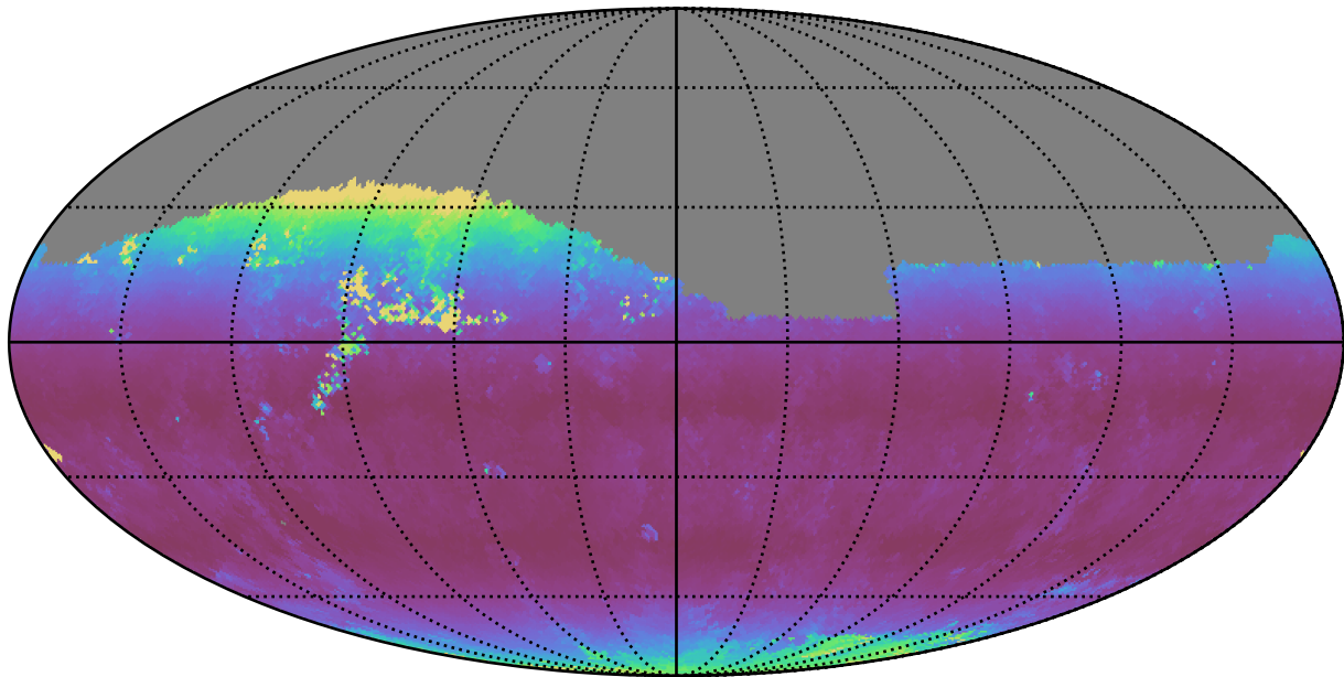
too_elab_r8_d3_griz_v3.4_10yrs Yr 1 i band: Median airmass
