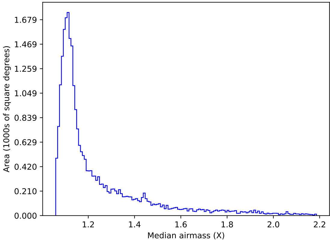
too_elab_r8_d3_griz_v3.4_10yrs Yr 1 i band: Median airmass
