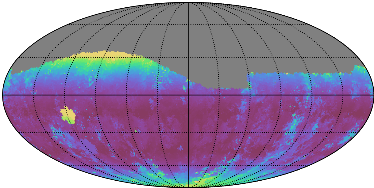
too_elab_r8_d3_griz_v3.4_10yrs Yr 1 g band: Median airmass
