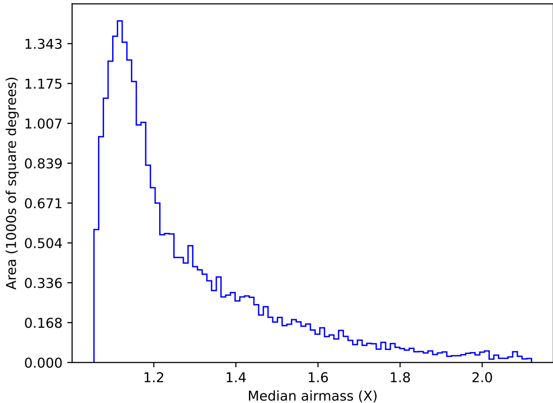
too_elab_r8_d3_griz_v3.4_10yrs Yr 1 g band: Median airmass
