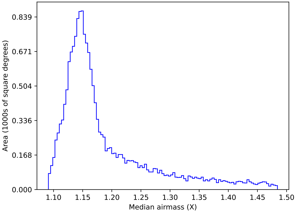
too_elab_r8_d3_griz_v3.4_10yrs WFD y band: Median airmass
