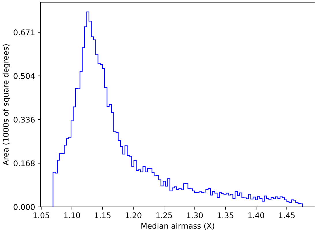
too_elab_r8_d3_griz_v3.4_10yrs WFD u band: Median airmass
