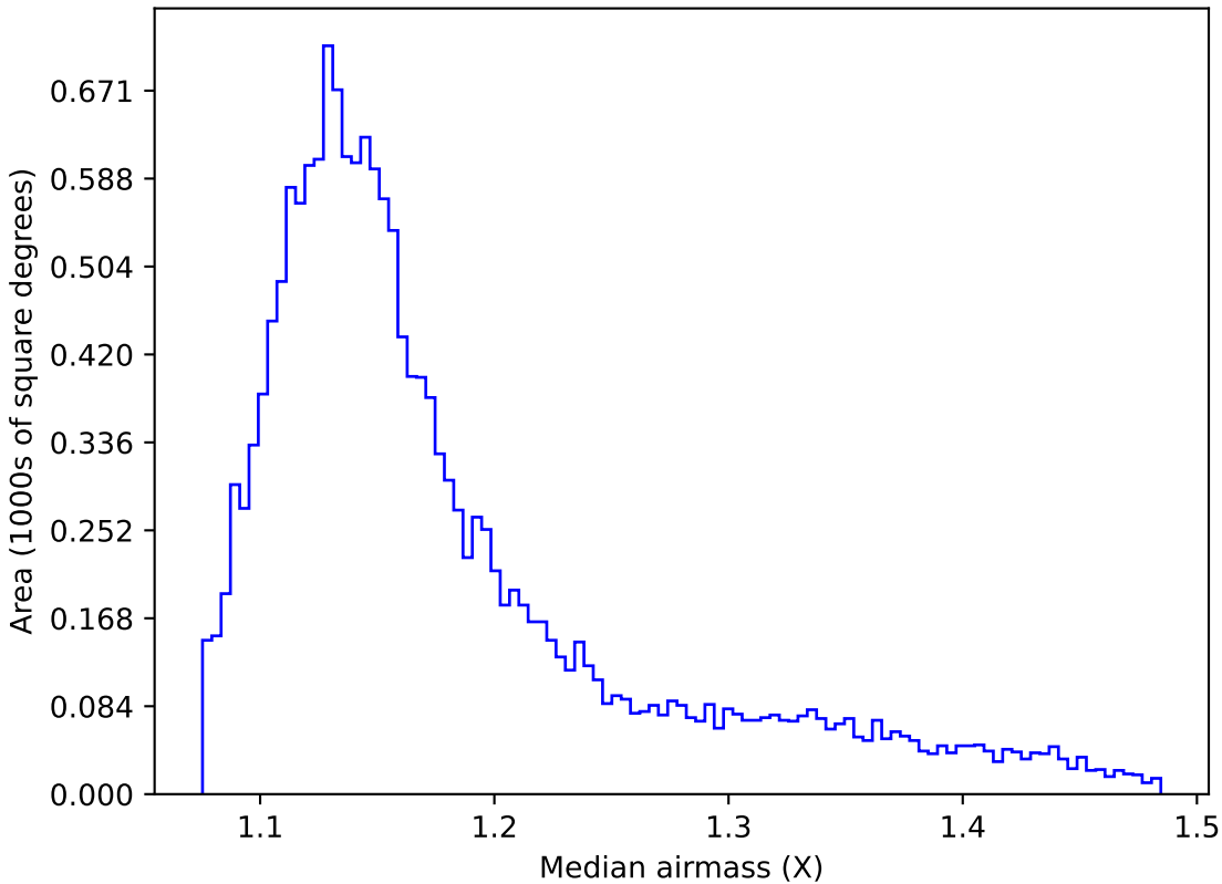
too_elab_r8_d3_griz_v3.4_10yrs WFD g band: Median airmass
