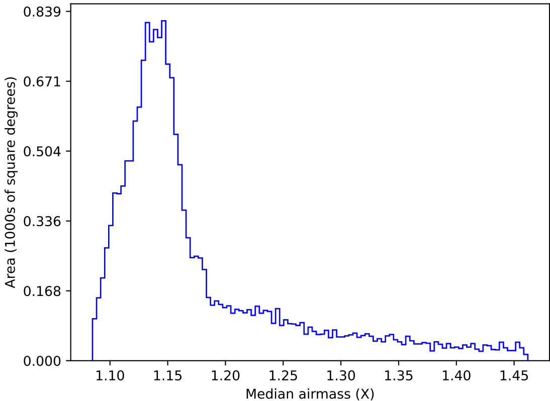
too_elab_r8_d3_griz_v3.4_10yrs WFD all bands: Median airmass
