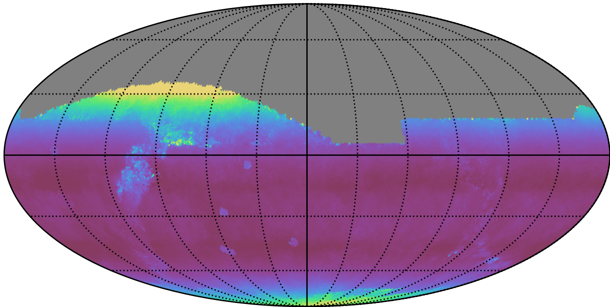
too_elab_r8_d3_griz_v3.4_10yrs All sky z band: Median airmass
