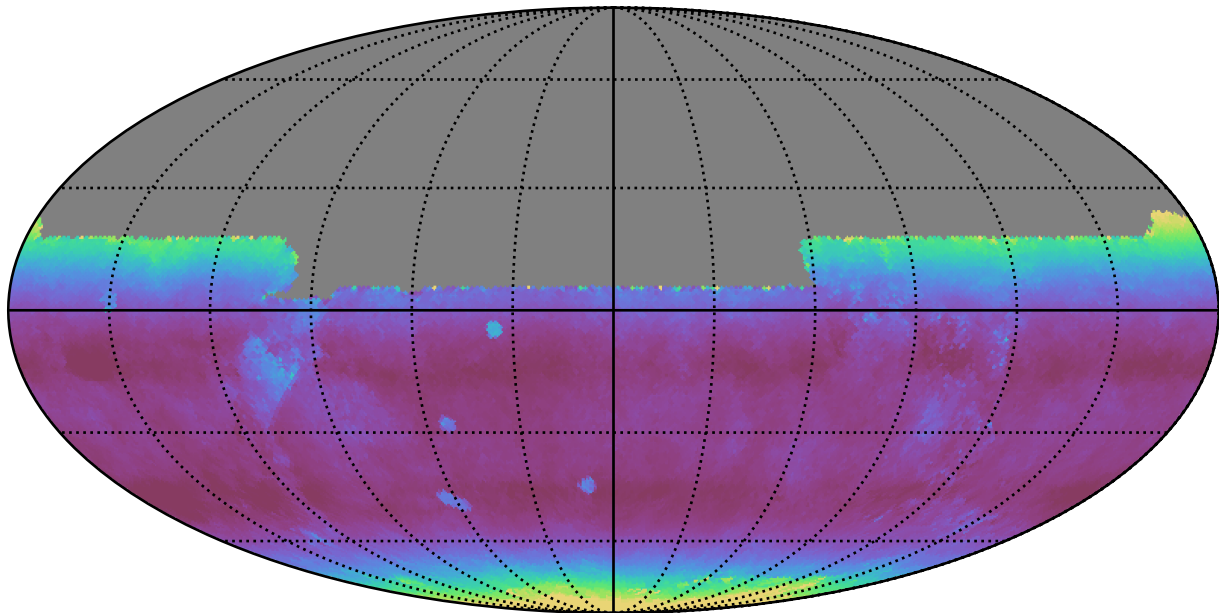
too_elab_r8_d3_griz_v3.4_10yrs All sky y band: Median airmass
