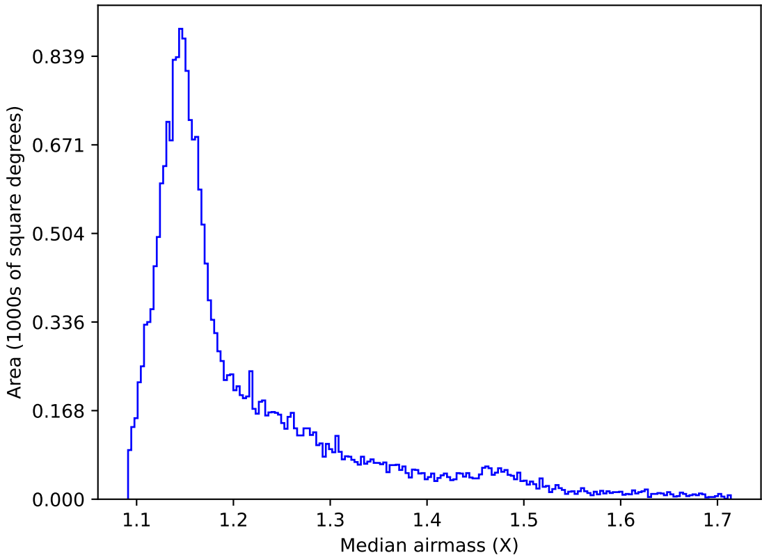
too_elab_r8_d3_griz_v3.4_10yrs All sky y band: Median airmass
