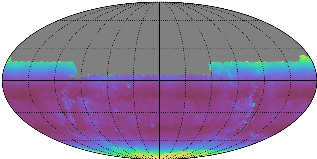
too_elab_r8_d3_griz_v3.4_10yrs All sky u band: Median airmass
