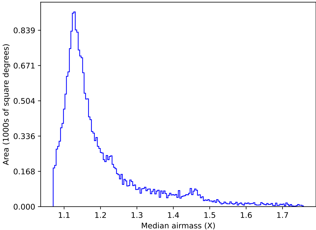
too_elab_r8_d3_griz_v3.4_10yrs All sky u band: Median airmass
