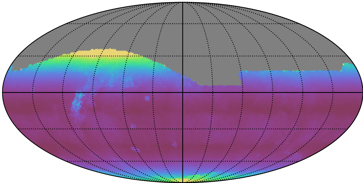
too_elab_r8_d3_griz_v3.4_10yrs All sky r band: Median airmass
