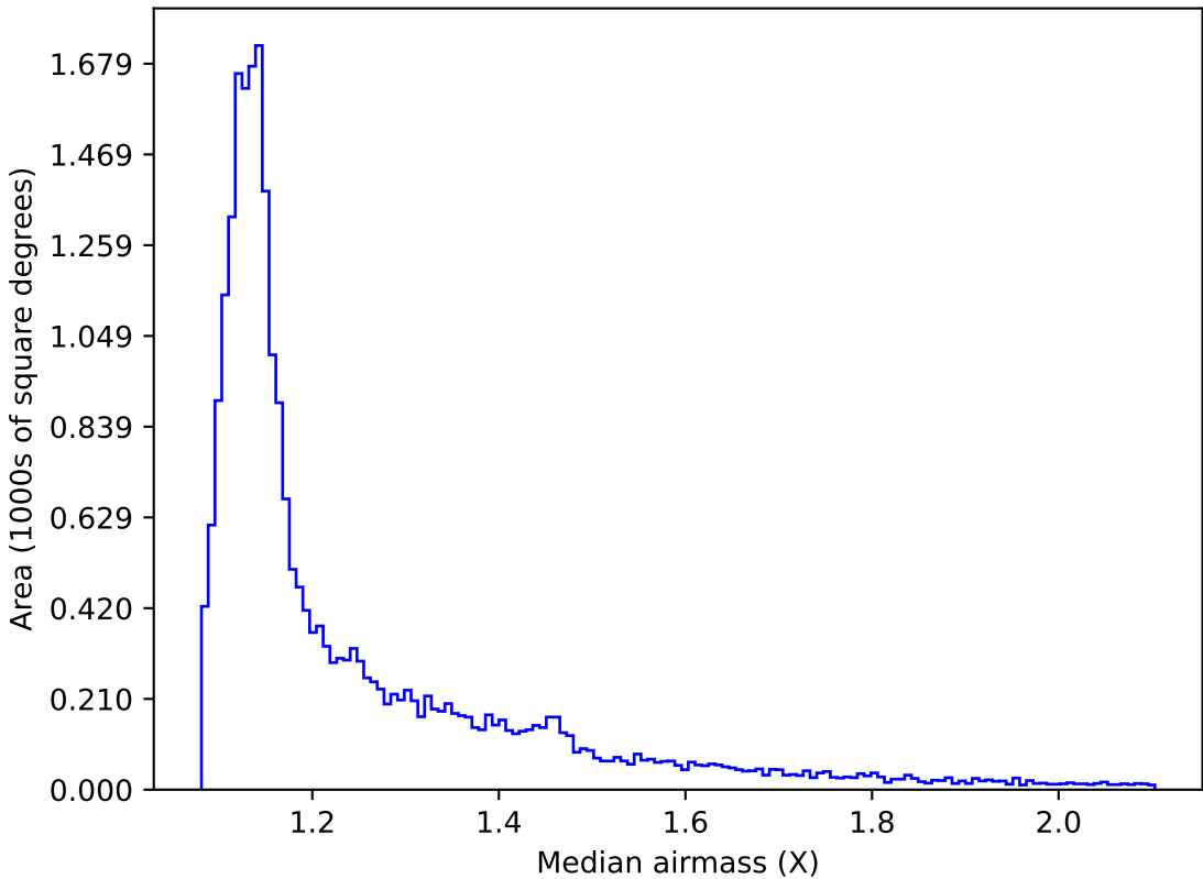
too_elab_r8_d3_griz_v3.4_10yrs All sky i band: Median airmass
