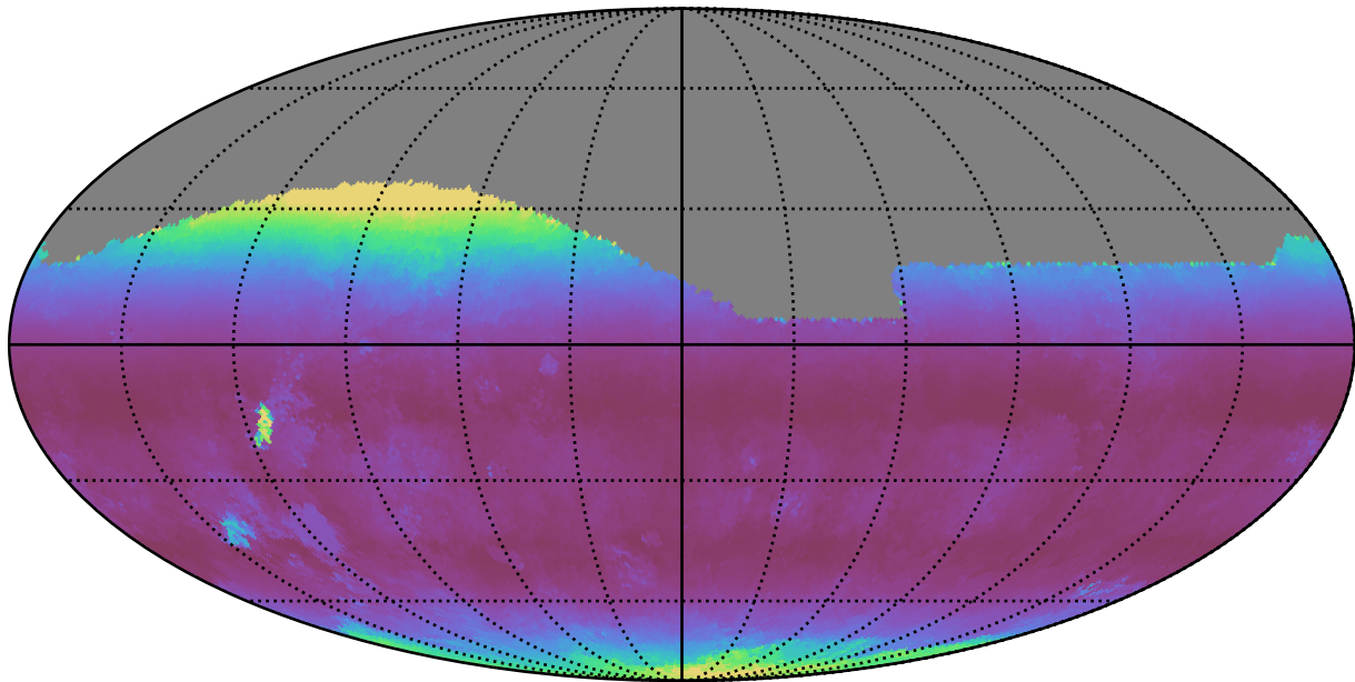
too_elab_r8_d3_griz_v3.4_10yrs All sky g band: Median airmass
