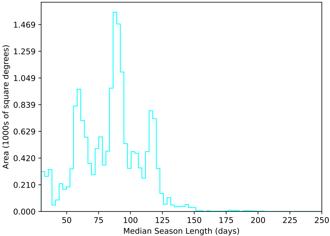
too_elab_r8_d3_griz_v3.4_10yrs WFD u band: Median Season Length
