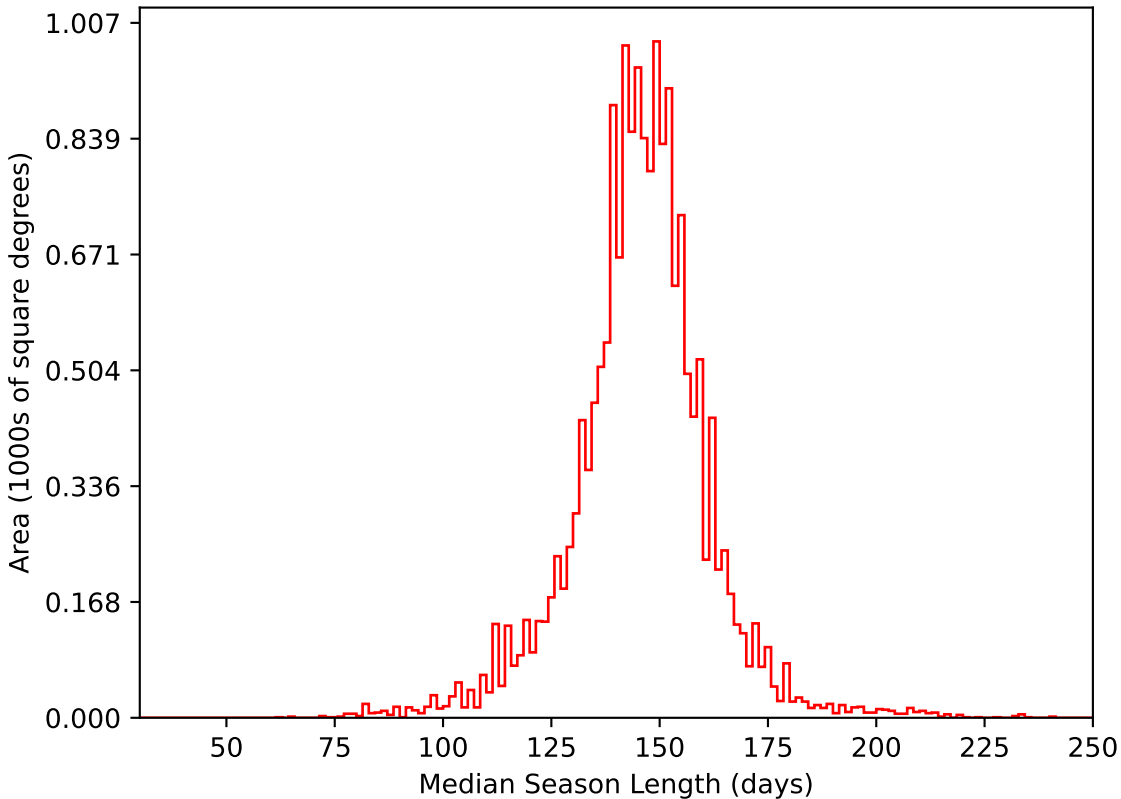
too_elab_r8_d3_griz_v3.4_10yrs WFD i band: Median Season Length
