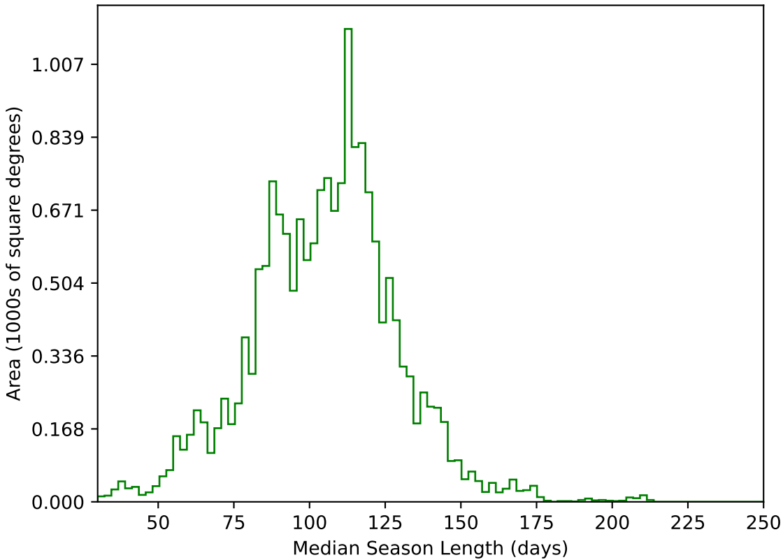
too_elab_r8_d3_griz_v3.4_10yrs WFD g band: Median Season Length
