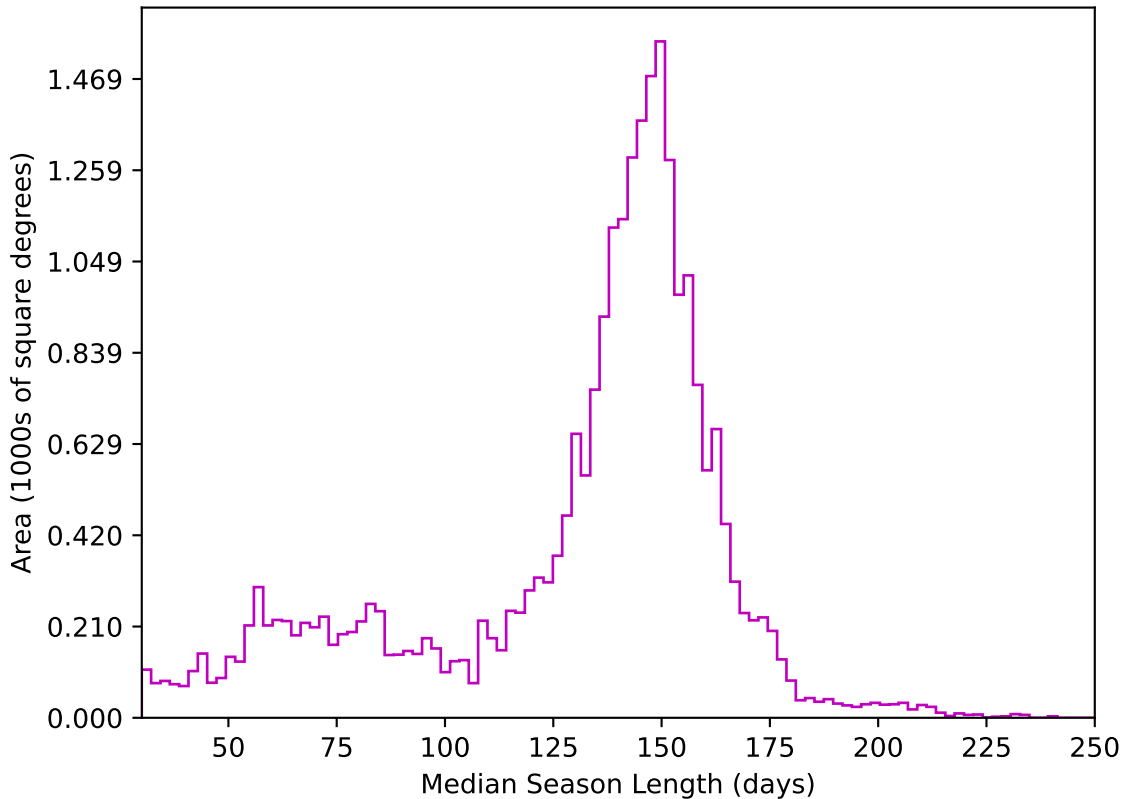
too_elab_r8_d3_griz_v3.4_10yrs All sky z band: Median Season Length
