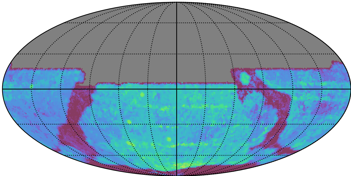
too_elab_r8_d3_griz_v3.4_10yrs All sky y band: Median Season Length
