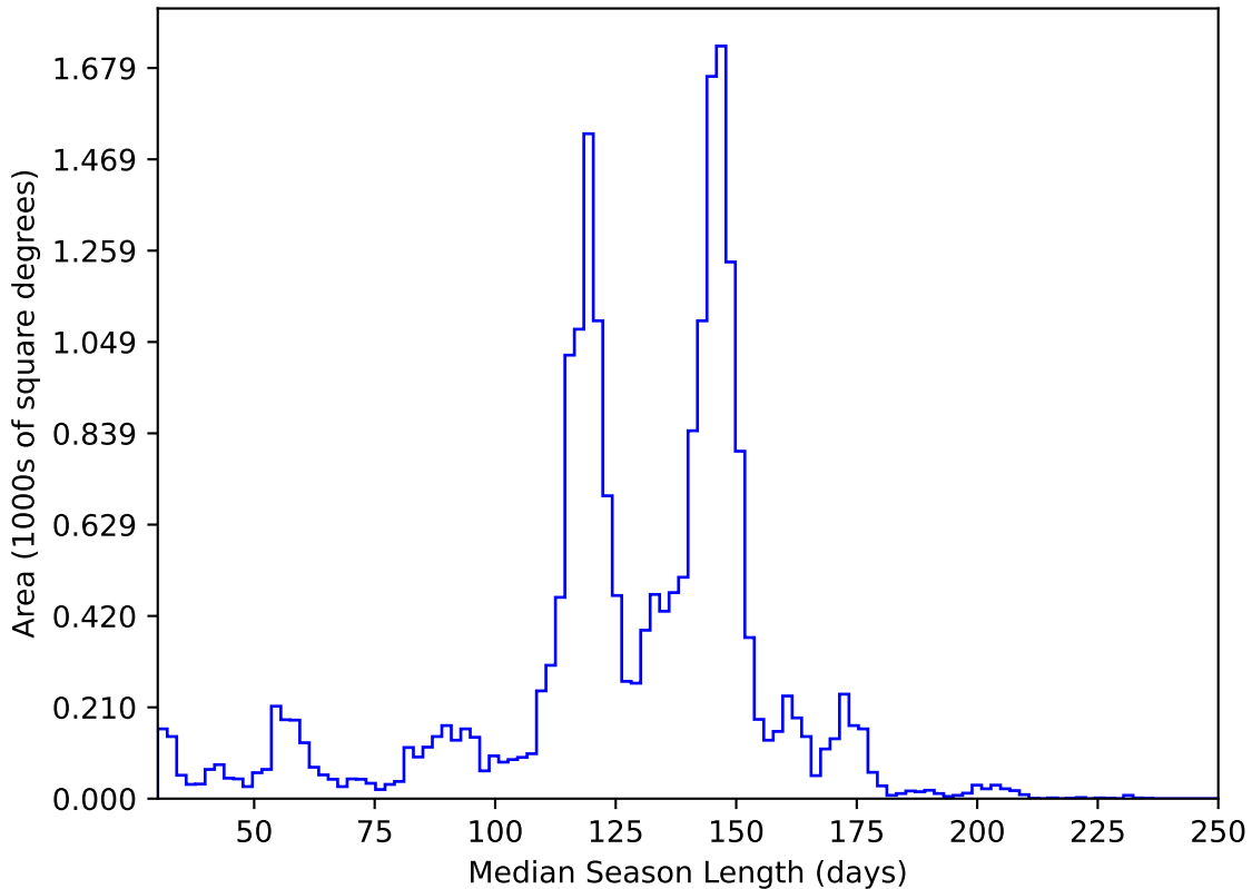
too_elab_r8_d3_griz_v3.4_10yrs All sky y band: Median Season Length
